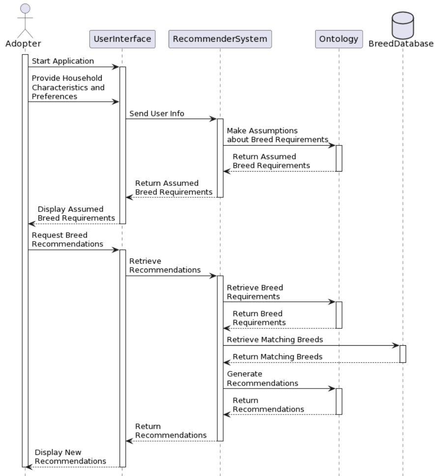
Activity Diagram - Alternate Flow #1
